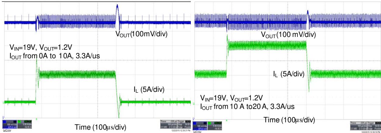
Figure 24. Load Transient from 0% to 50% Load Current
