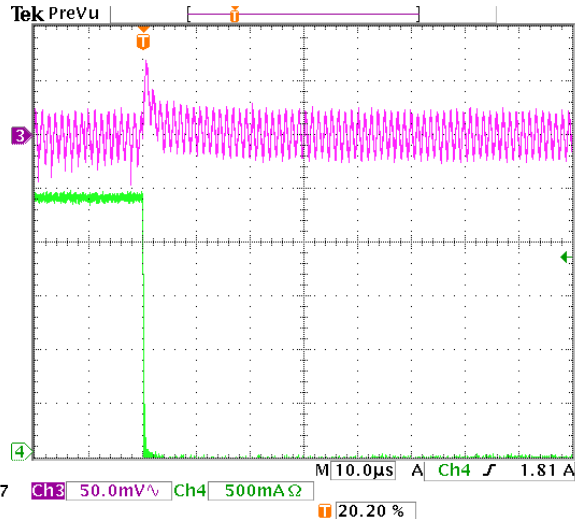
Output Load Release Response
