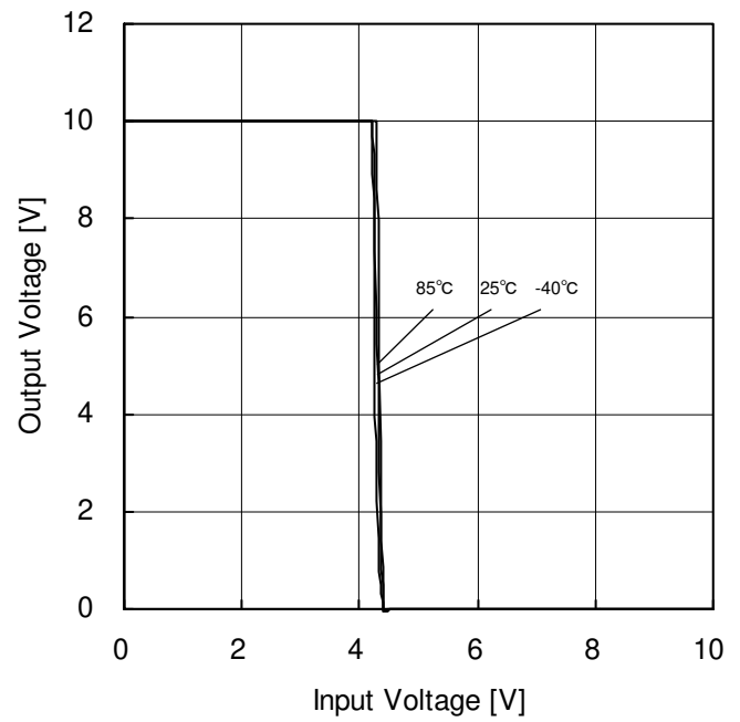
Figure 2. Output Voltage vs Input Voltage (V DD =10V / V SS =0V)
