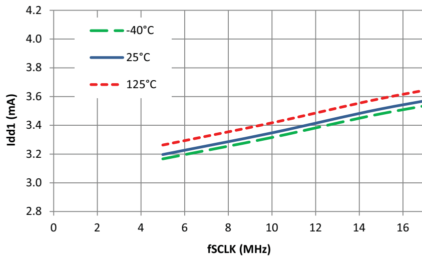
Figure 7: Power Supply Current vs. SPI Clock Frequency
