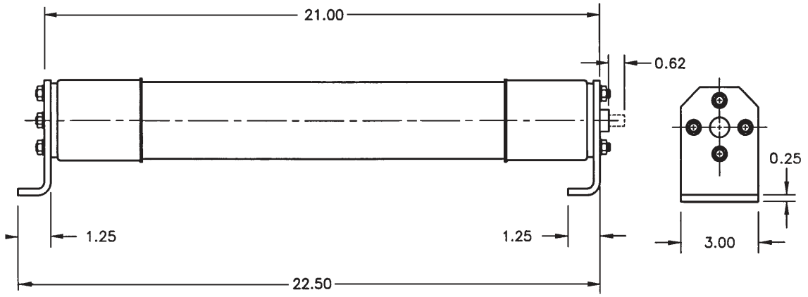
Figure 1 Dimensions - in
