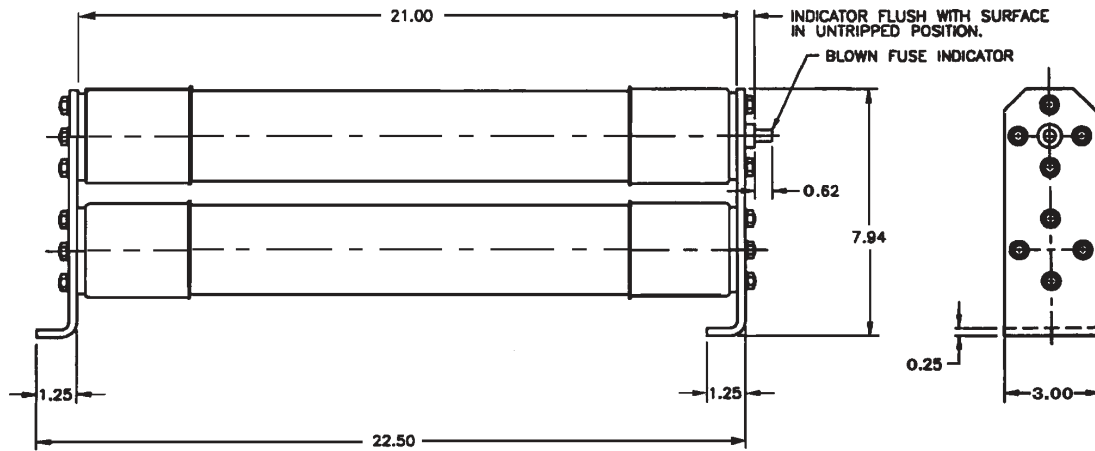
Figure 2 Dimensions - in
