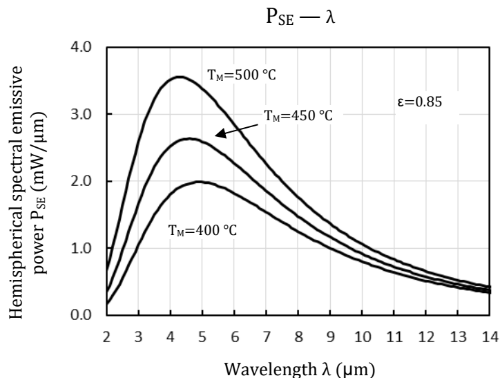
Hemispherical spectral emissive power of EMIRS200 chip surface with a typical emissivity (mean from 2 to 14 \mu\text{m} ) of \epsilon = 0.85
