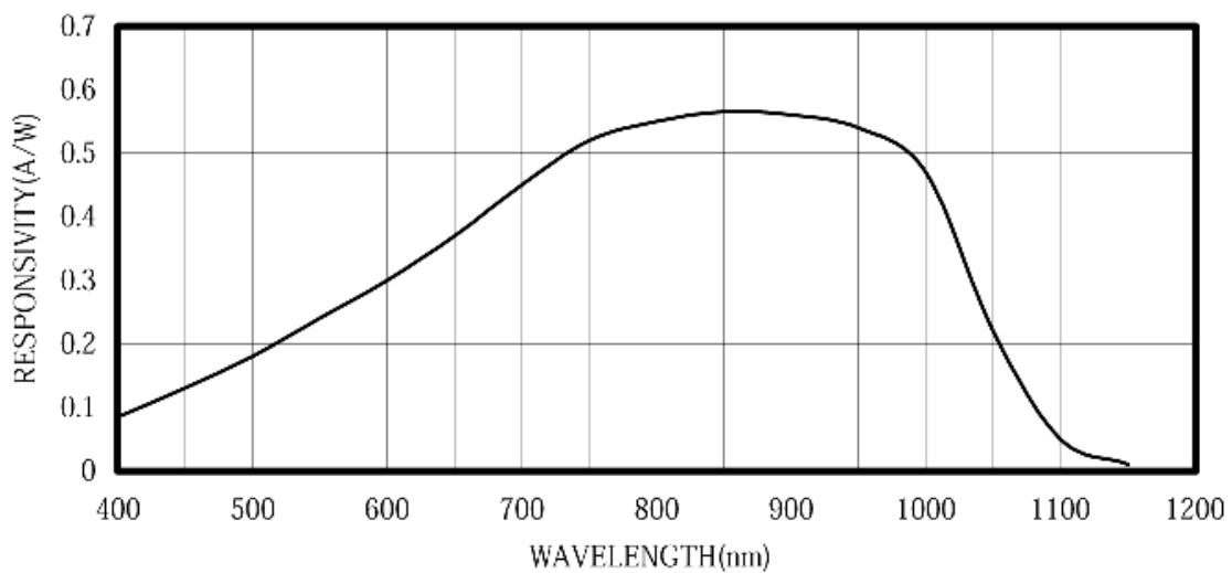
RESPONSIVITY
