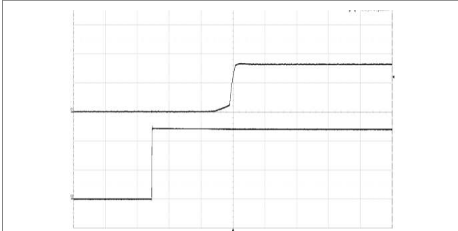
Start-up enabled by connecting V_i at: T_{P1} = +25^\circ\text{C} , V_i = 24\text{ V} , I_o = 4.5\text{ A} electronic load. Top trace: output voltage (2 V/div.). Bottom trace: input voltage (10 V/div.). Time scale: (2 ms/div.).
