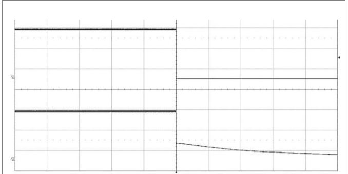
Output disabled by removing V_I at: T_{P1} = +25^{\circ}\text{C} , V_I = 24\text{ V} , I_O = 2.5\text{ A} resistive load. Top trace: output voltage (5 V/div.). Bottom trace: input voltage (10 V/div.). Time scale: (200 ms/div.).
