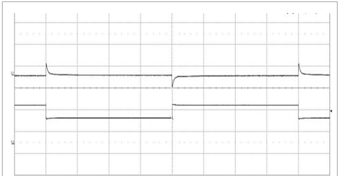
Output voltage response to load current step-change (1.25-1.875-1.25 A) at: T_{P1} = +25^{\circ}\text{C} , V_I = 24\text{ V} . Top trace: output voltage (500 mV/div.). Bottom trace: load current (1 A/div.). Time scale: (2 ms/div.).
