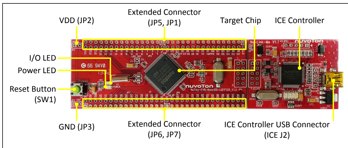
Figure 2-1 NuTiny-SDK-NANO100 (PCB Board)
