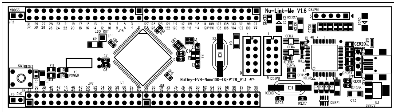
Figure 2-2 NuTiny-SDK-NANO100 PCB Placement
