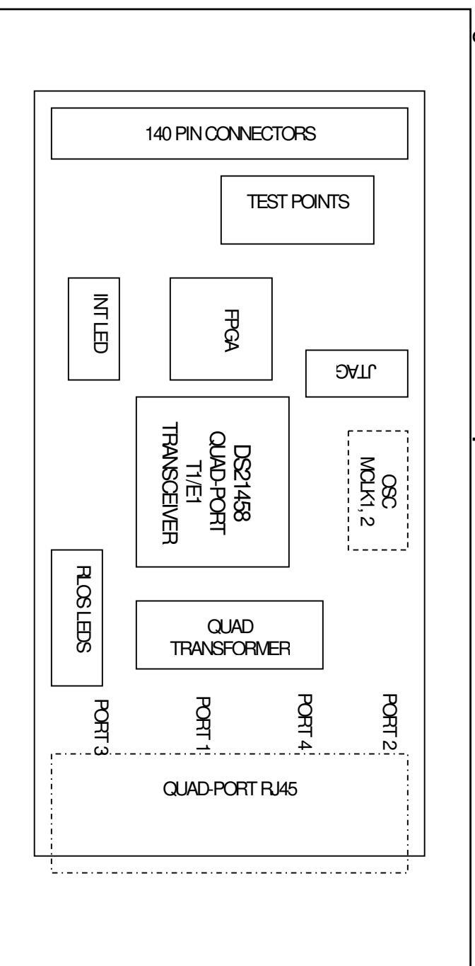
Figure 2. DS21458 Resource Card Floorplan
