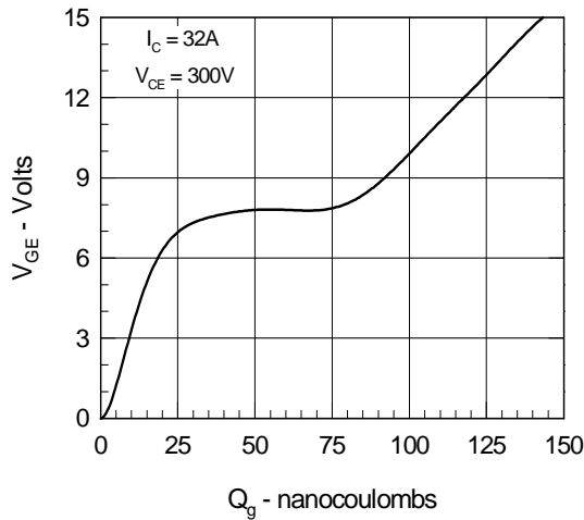
Fig. 9. Gate Charge
