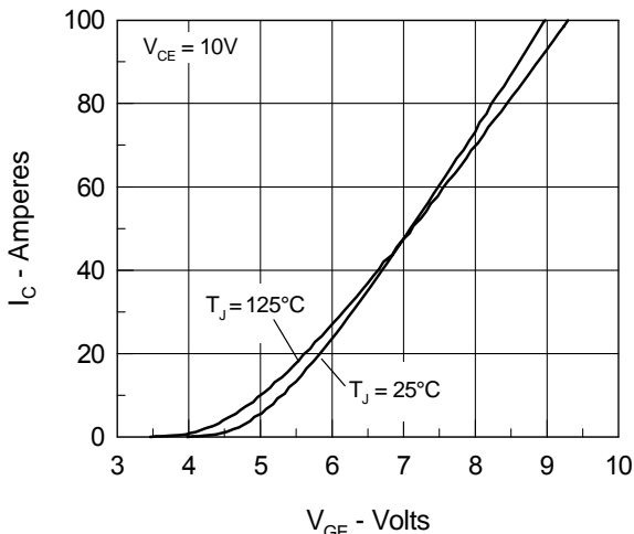
Fig. 5. Admittance Curves
