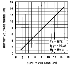
Open Voltage Swing vs Supply Voltage
