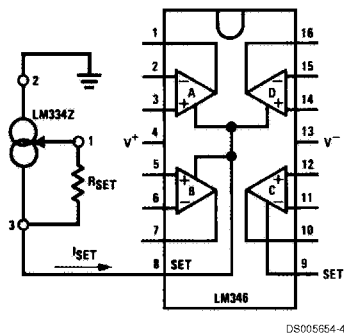
Current Source Biasing with Temperature Compensation
