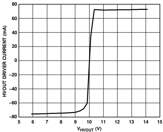
Figure 29. HVOUT VHH Current Limit; V_{HH} = 10.0\text{ V} ; V_{HVOUT} Swept from -5.9\text{ V} to +14.1\text{ V}
