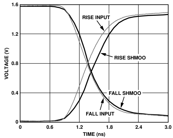
Figure 32. Comparator Shmoo, 1.5 V Input, 1.0 ns (10% to 90%) Input, 50 Ω Terminated
