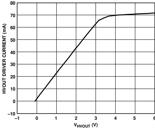
Figure 28. HVOUT VH Current Limit; V_H = -0.1\text{ V} ; V_{HVOUT} Swept from -0.1\text{ V} to +6.0\text{ V}
