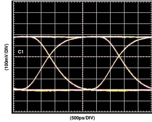
Figure 60. Eye Diagram, 400 Mbps, PRBS31; VH = 1.0 V, VL = 0.0 V
