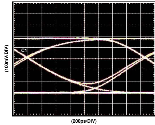
Figure 61. Eye Diagram, 600 Mbps, PRBS31; VH = 1.0 V, VL = 0.0 V
