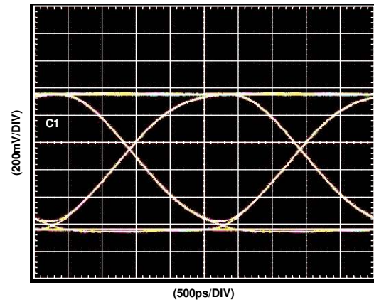
Figure 62. Eye Diagram, 400 Mbps, PRBS31; VH = 2.0 V, VL = 0.0 V
