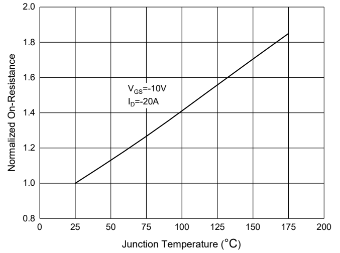
Fig. 4 - R_{DS(ON)} - Temperature
