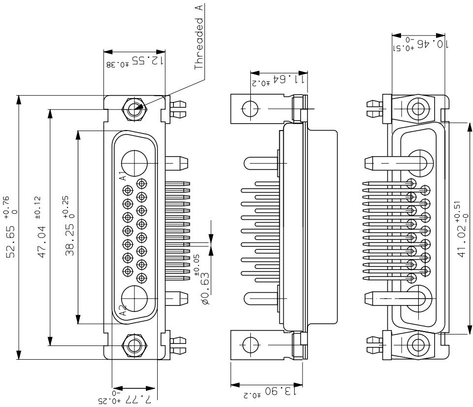
LAYOUT DIMENSIONS (after plating)
