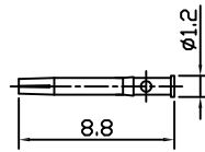
Pin contact
