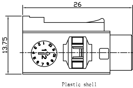
Plastic shell
