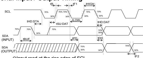
Input read at the rise edge of SCL OData output in sync with the fall of SCL Figure 2-(a). Serial Input / Output timing
