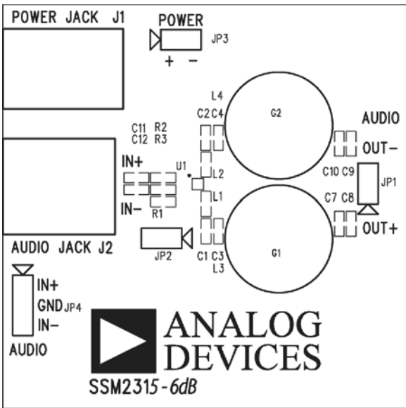
Figure 6. Top Silkscreen
