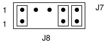
Figure 2-4. CY3209FirstEx Jumper Settings
