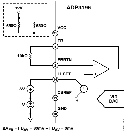
Figure 4. Positioning Voltage
