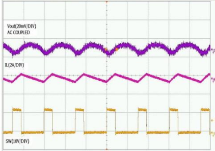
Time -2µs/div
