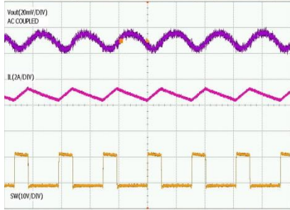
Time -2µs/div
