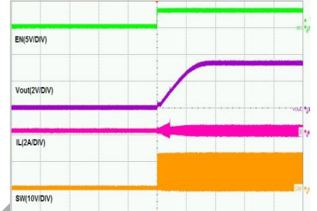
Time -10ms/div
