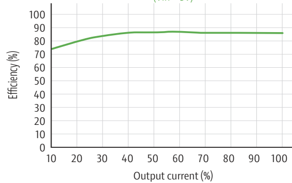
Efficiency vs output load (Vin = 5V)
