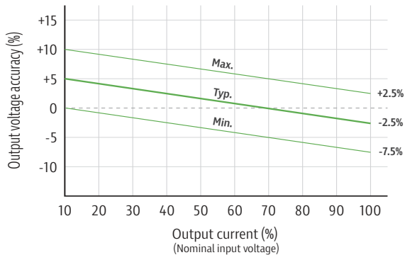
Output regulation curve
