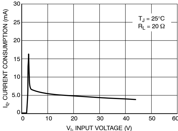
Figure 16. Current Consumption vs. Input Voltage, 3.3 V Version
