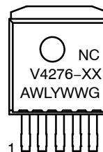
NCV4276 D 2 PAK 5-PIN DS SUFFIX CASE 936A
