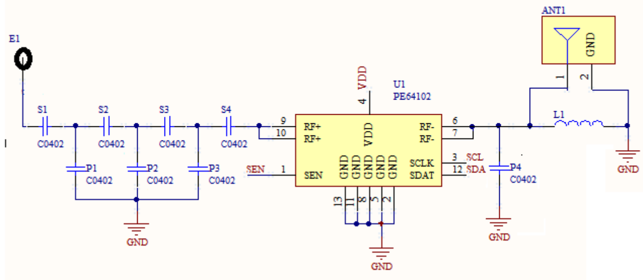
Figure 25. Matching Circuit, PE64102 and DTA01 Antenna.
