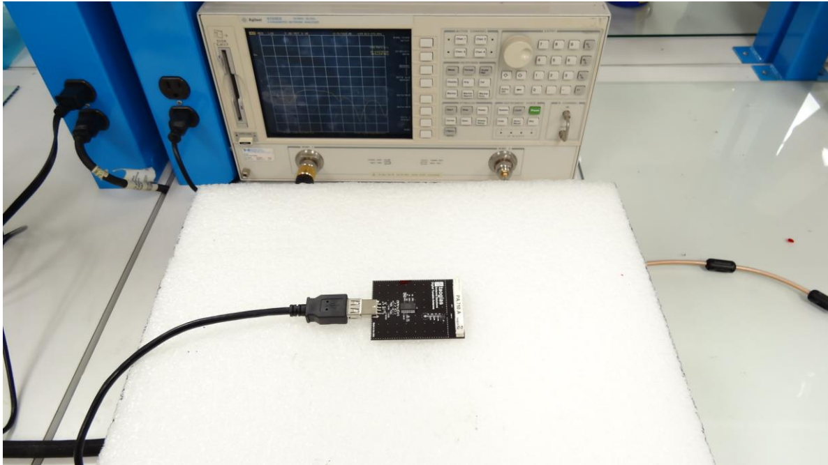
Figure 1. Impedance test.
