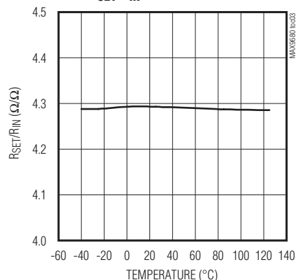
R SET /R IN vs. TEMPERATURE
