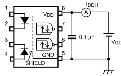
Fig. 12.1.4 IDDH Test Circuit
