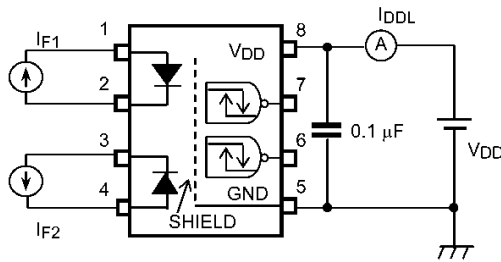
Fig. 12.1.3 IDDL Test Circuit
