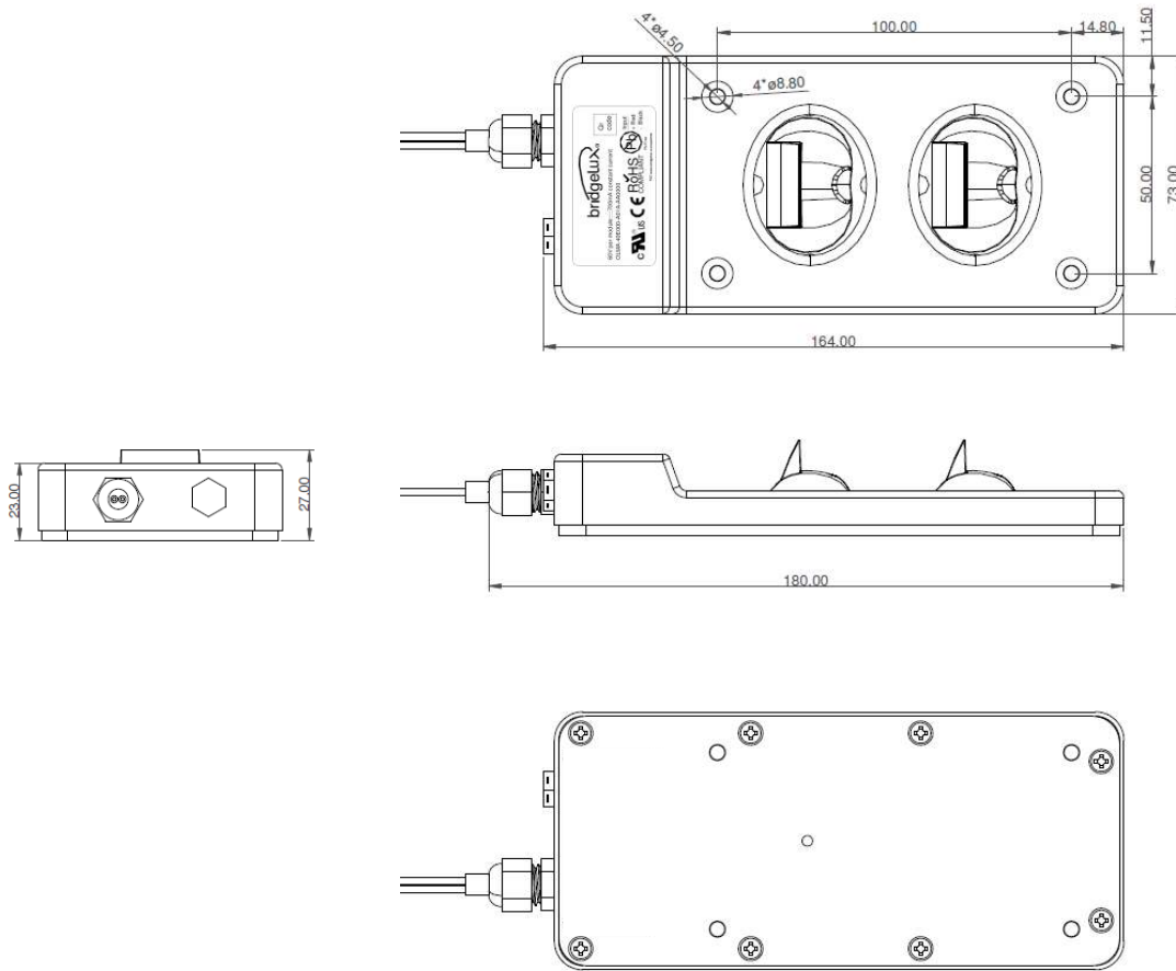
Figure 5: Mechanical Dimensions
