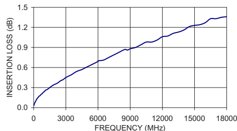
141-24SM+ INSERTION LOSS
