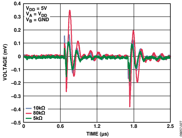
Figure 27. Digital Feedthrough
