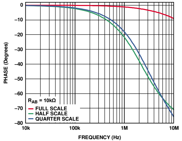
Figure 18. Normalized Phase Flatness vs. Frequency
