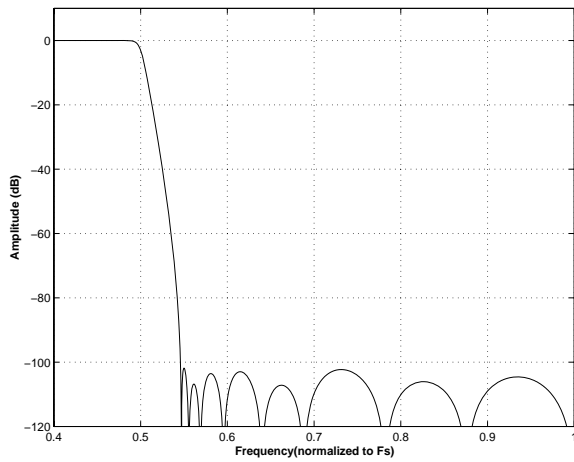
Figure 31. Single-Speed Stopband Rejection
