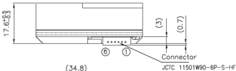
[ Marking portion ]
