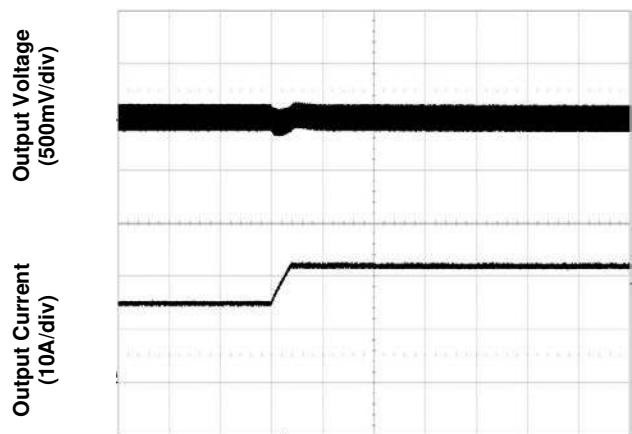
Figure 6. Transient Load Response (typical V_{in} , load current steps from 50% to 75% at a slew rate 0.1A/ \mu s, 1,000 \mu F external output capacitance)
