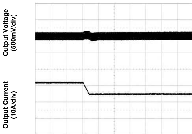
Figure 5. Transient Load Response (typical V_{in} , load current steps from 75% to 50% at a slew rate 0.1A/ \mu s, 1,000 \mu F external output capacitance)
