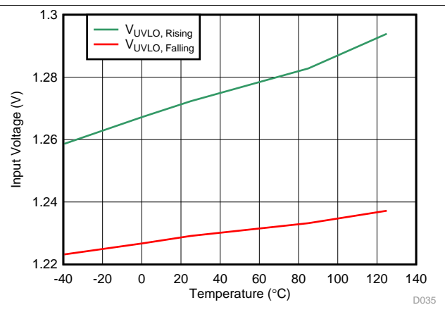
Figure 46. UVLO V_{IN} Rising and Falling Thresholds vs Temperature
