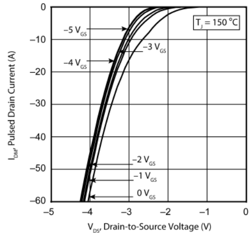
Figure 10 • I_{DM} vs. V_{DS} 3 rd Quadrant Condition
