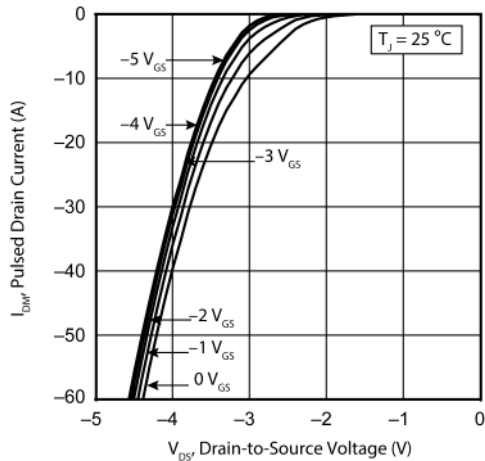
Figure 9 • I_{DM} vs. V_{DS} 3 rd Quadrant Condition
