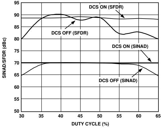
Figure 24. SINAD/SFDR vs. Clock Duty Cycle
