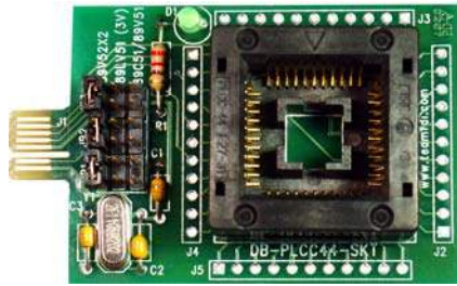
Board Dimensions 2.505" x 1.560"
