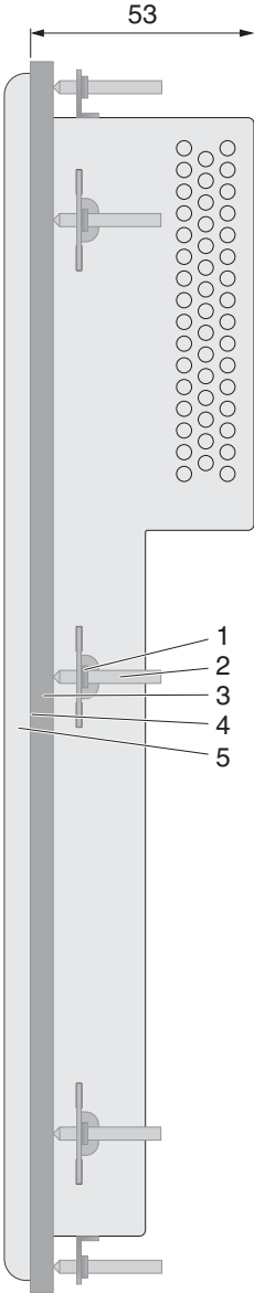
Figure 2-18 Side view, mounting depth (dimensions in mm)
