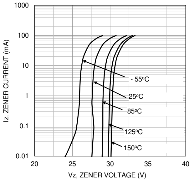
Figure 7. Zener Current vs. Zener Voltage
