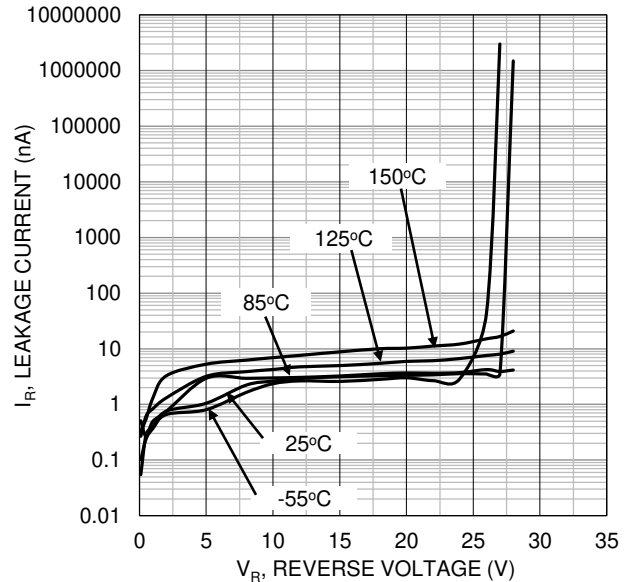
Figure 6. Leakage Current vs. Reverse Voltage
