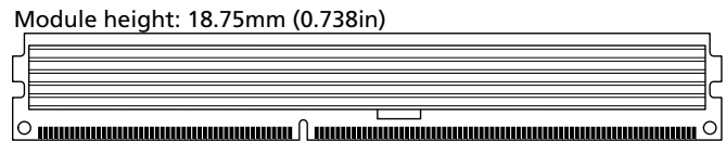
Figure 1: 240-Pin RDIMM (MO-269 R/C N)
