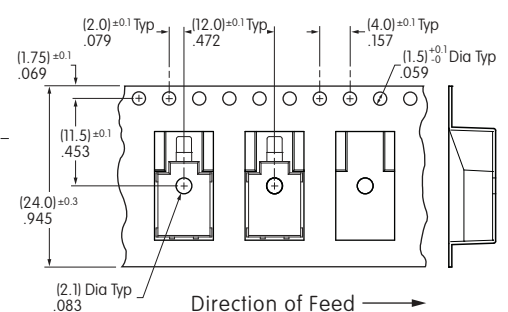
Tape Dimensions
