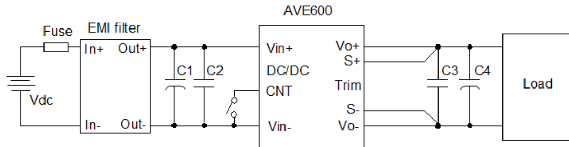
Figure 15 Typical application
