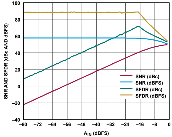
Figure 51. Single-Tone SFDR and SNR vs. A_{IN} at f_{IN} = 5.4 GHz
