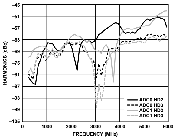
Figure 62. Harmonics (HD2 and HD3) vs. Frequency with A_{IN} = -1 dBFS
