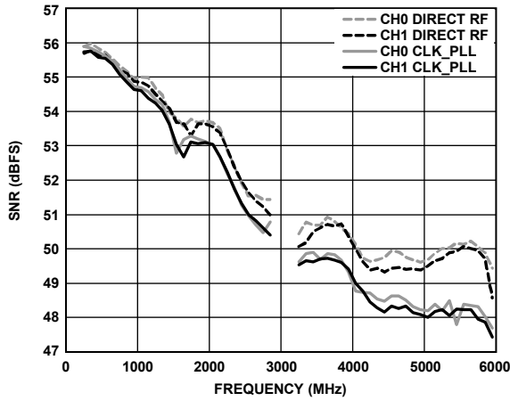
Figure 61. SNR vs. Frequency with A_{IN} = -1 dBFS Between Direct External RF Clock = 6 GHz and PLL Clock Multiplier Enabled with Reference Input of 125 MHz
