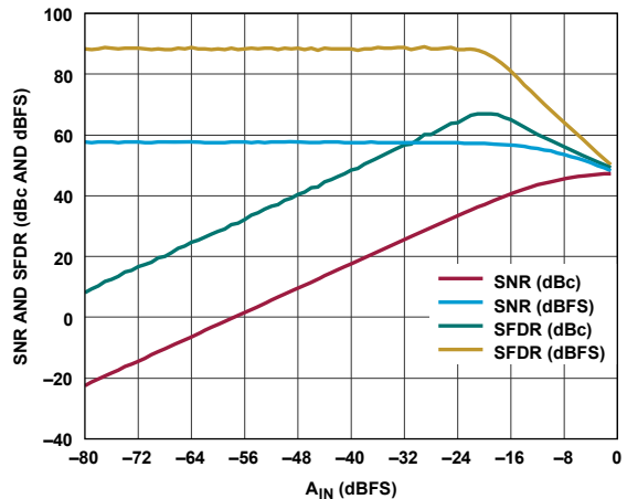
Figure 53. Single-Tone SFDR and SNR vs. A_{IN} at f_{IN} = 7.2 GHz
