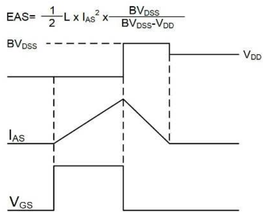
Figure 12. EAS Waveform
