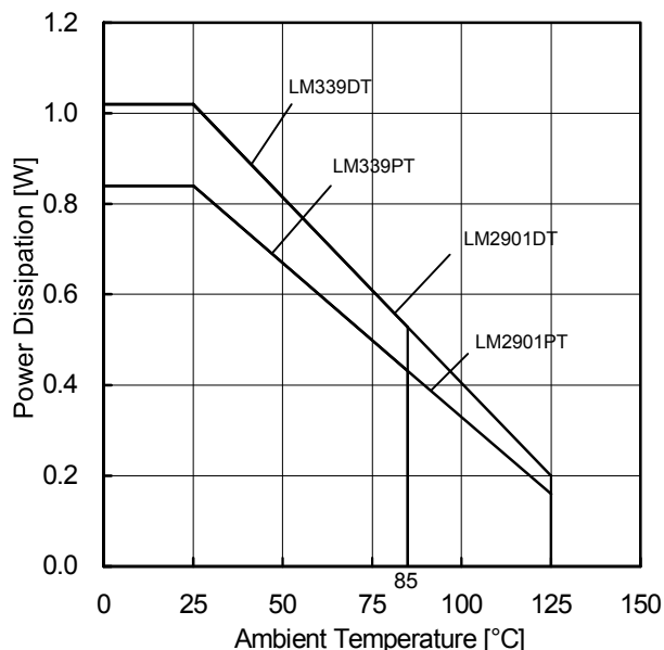
Figure 25. Power Dissipation vs Ambient Temperature (Derating Curve)
