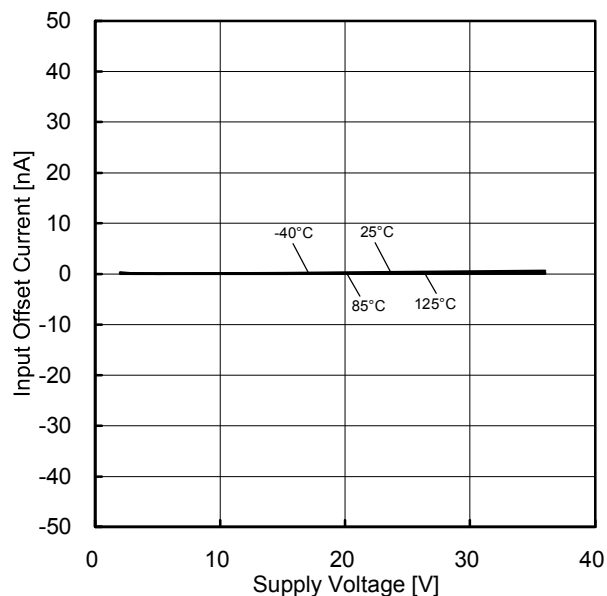
Figure 36. Input Offset Current vs Supply Voltage
