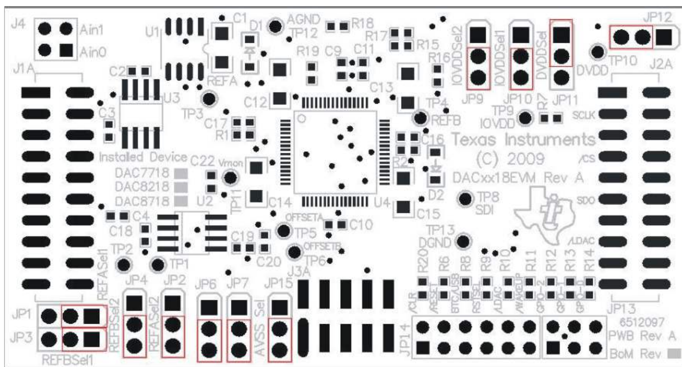
Figure 2. DAC7718EVM Default Jumper Locations for Bipolar Mode
