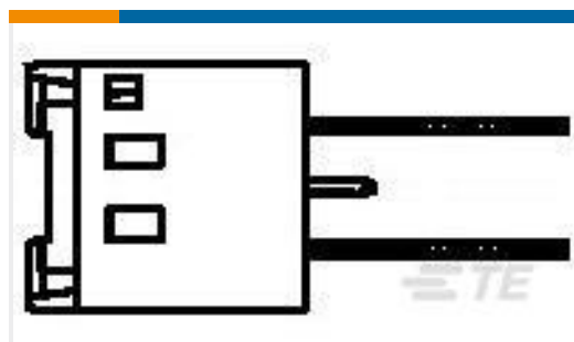
TE Part #1-178313-5 Header Assembly: Wire-to-Board, 15A, gold or tin plated
