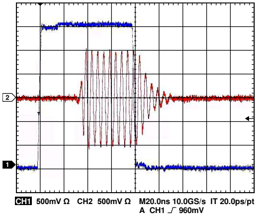
Figure 23. ENBL Time Domain Response
