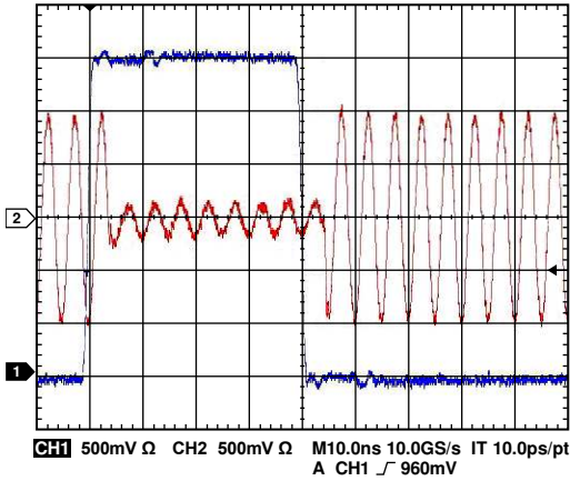
Figure 22. Gain Step Time Domain Response
