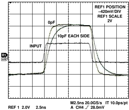
Figure 24. Pulse Response to Capacitive Loading, Gain -4 dB
