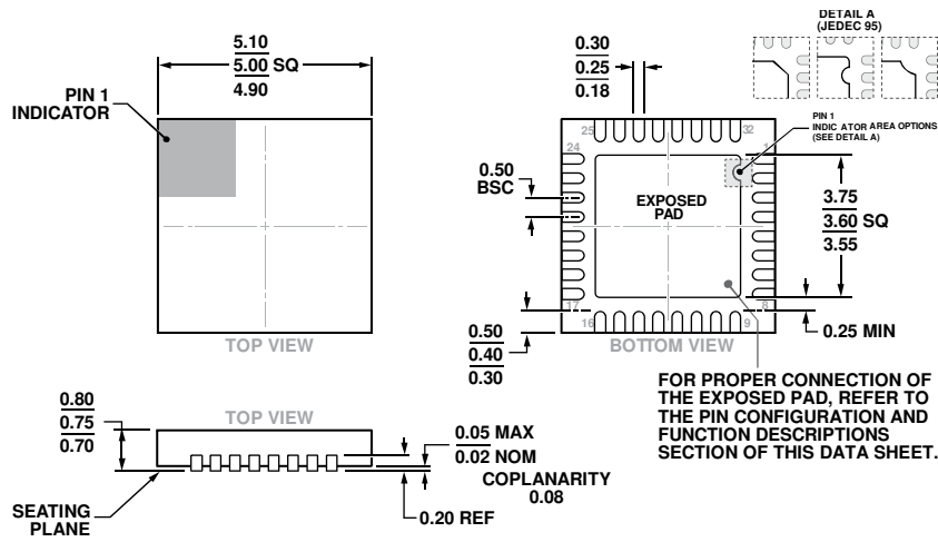
Figure 34. 32-Lead Lead Frame Chip Scale Package [LFCSP] 5 mm × 5 mm Body, and 0.75 mm Package Height (CP-32-12)
