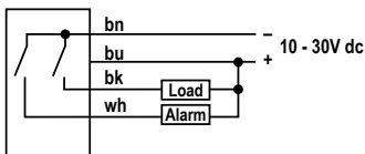
NPN (Sinking) Outputs Alarm Hookup
