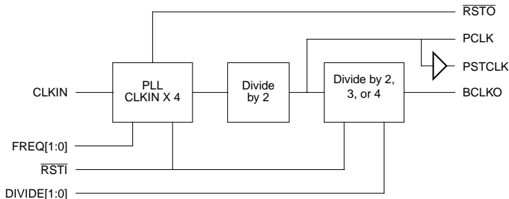
Figure 7-1. PLL Module Block Diagram
